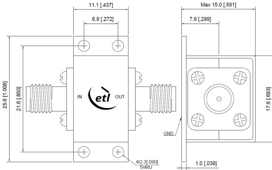
Dimensions (mm)
